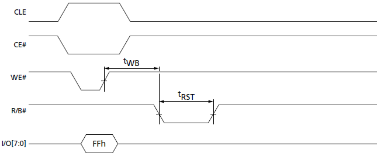
Figure 27 : Reset operation timing
