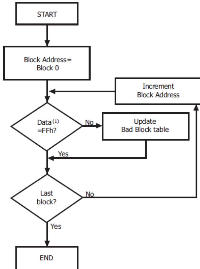
Figure 33 : Bad Block Management Flowchart
