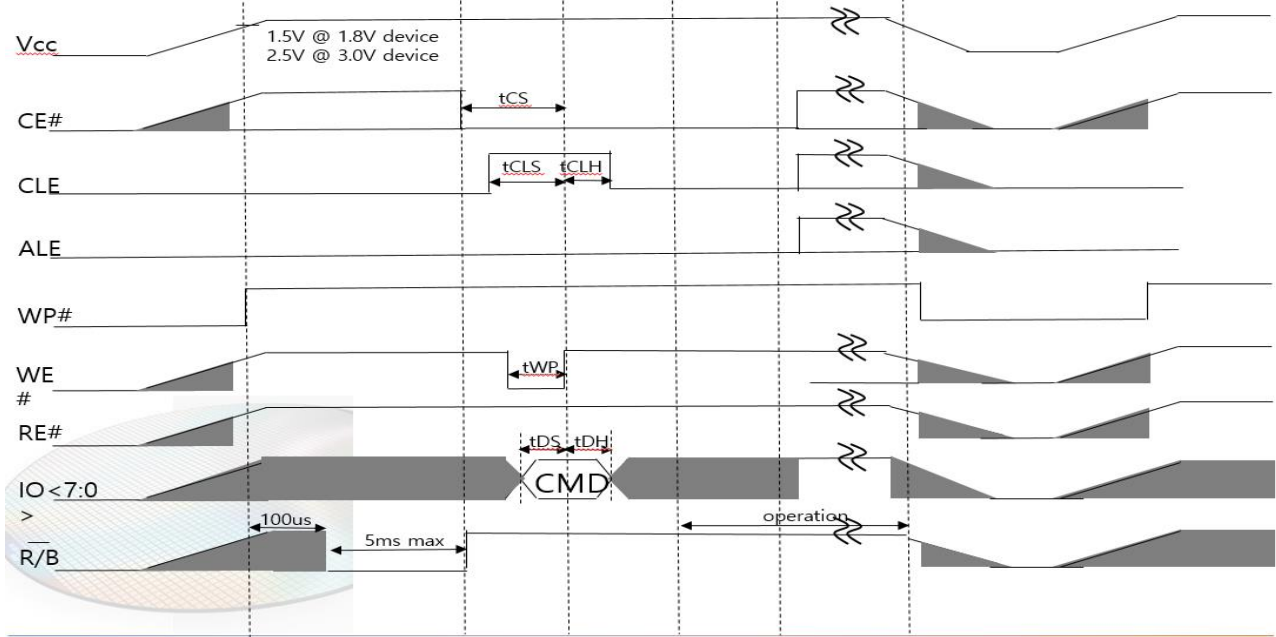
Figure 31 : Power up time sequence
